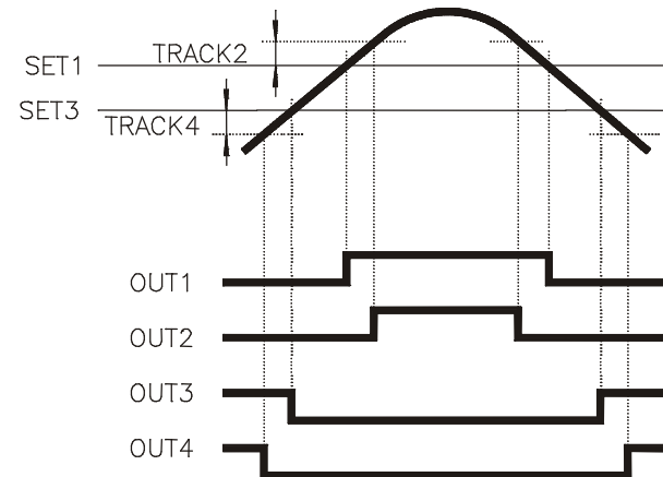
Fig 2. Tracking setpoints
