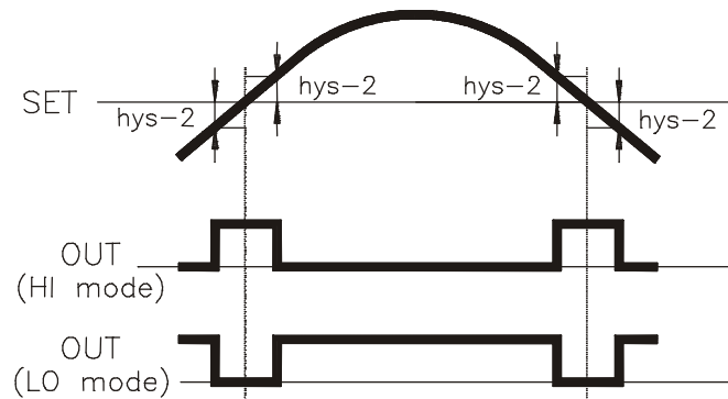
Fig 1. Symmetrical hysteresis
